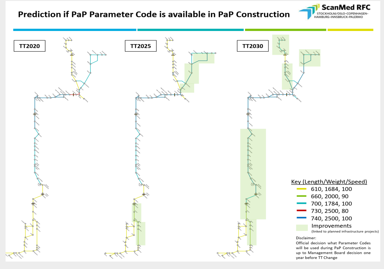
Figure 4: Infrastructure improvements by 2030 - ScanMed RFC, source [23]
