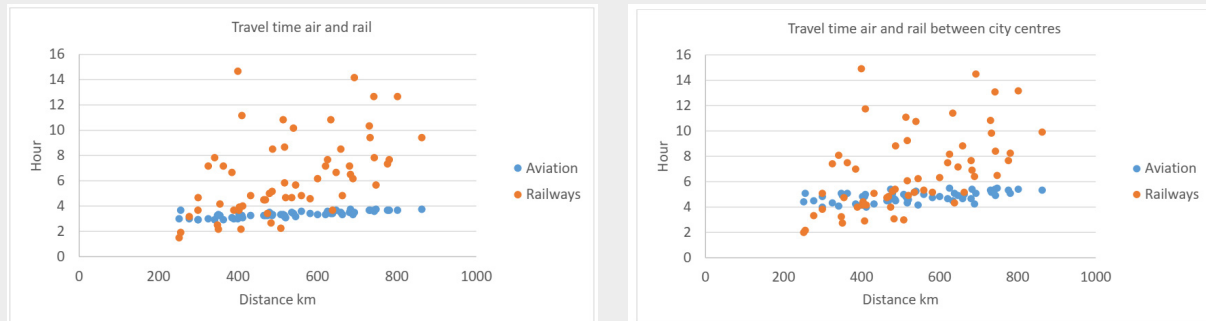
Figure 20: Travel time between airports and railway stations (left) or between city centres (right) of 58 city pairs, source [16]
